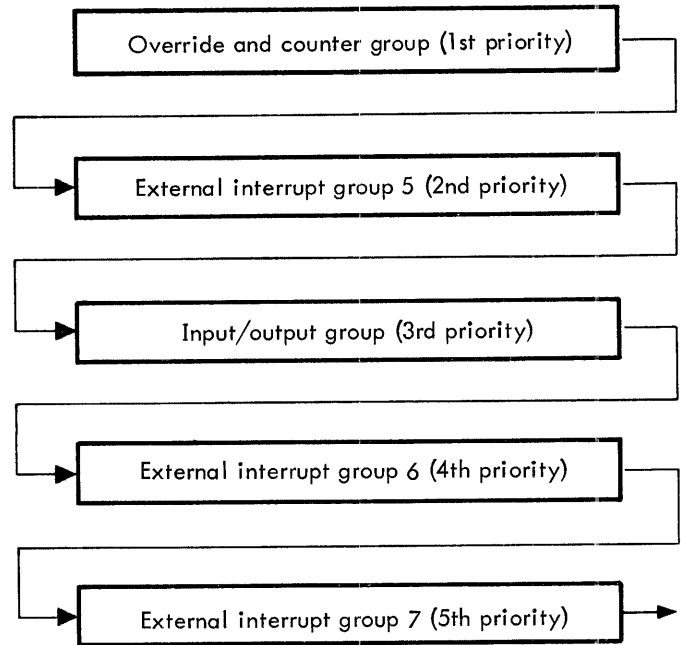
Figure 4. Interrupt Priority Chain
