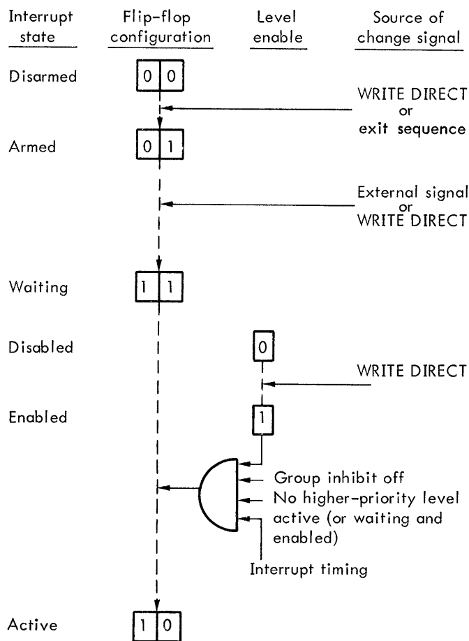
Figure 3. Interrupt Level Operation
