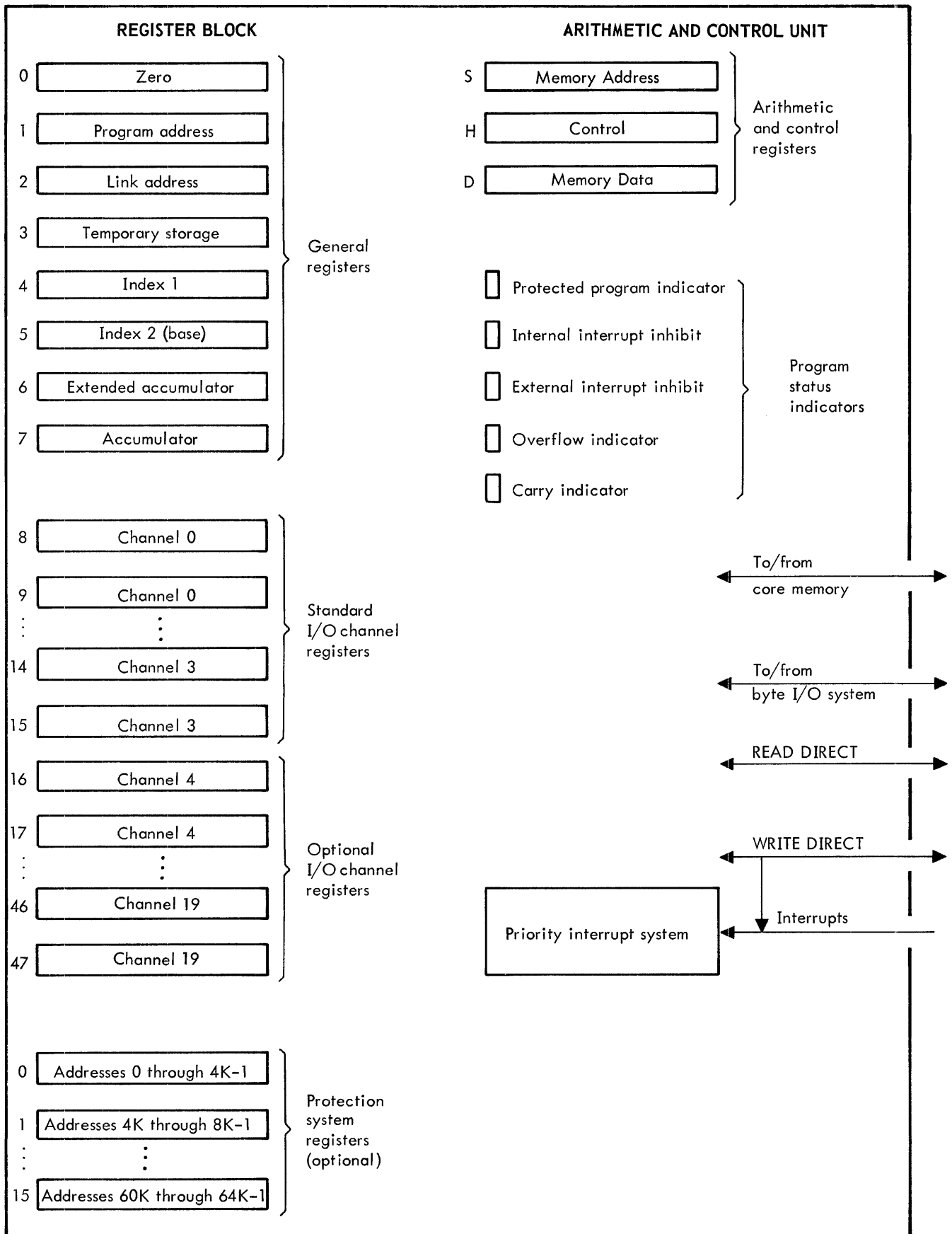
Figure 2. SIGMA 2 Central Processing Unit
