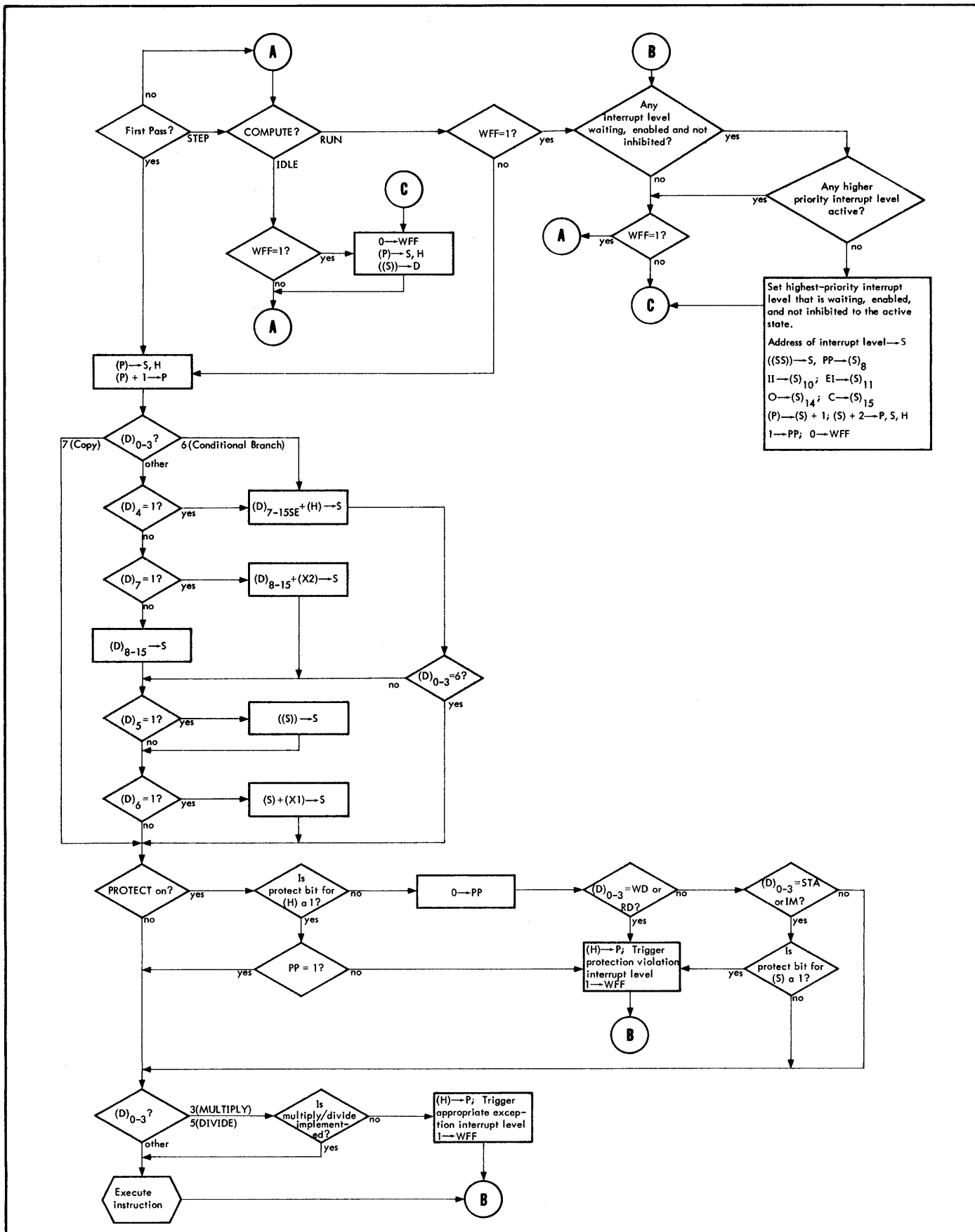
Figure 7. SIGMA 2 Instruction Execution Diagram
