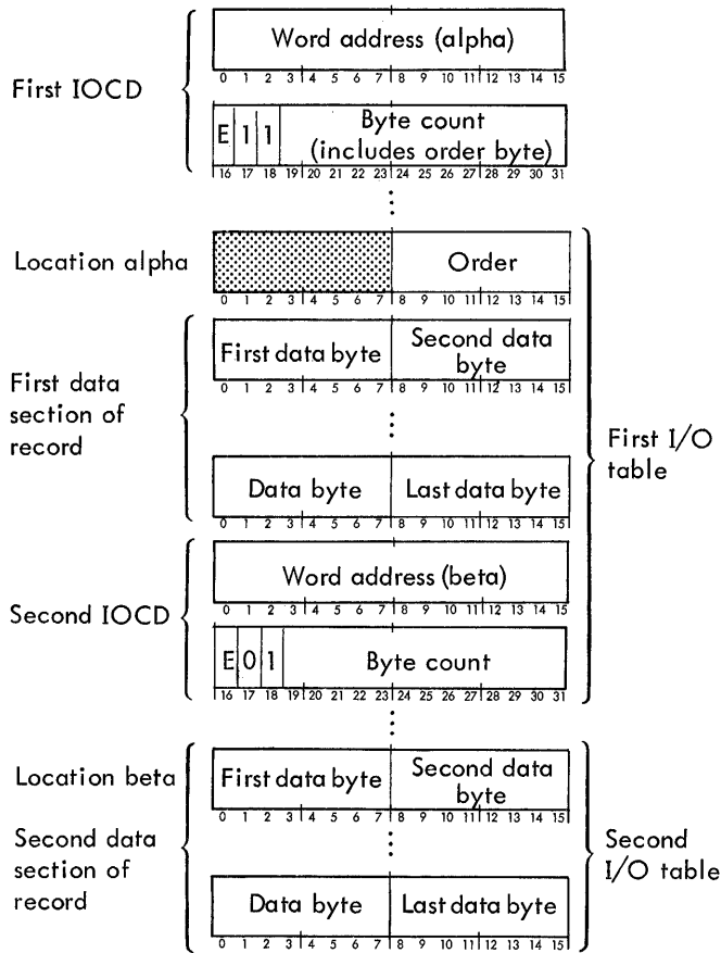
Figure 5. I/O Control Doublewords and I/O Tables
