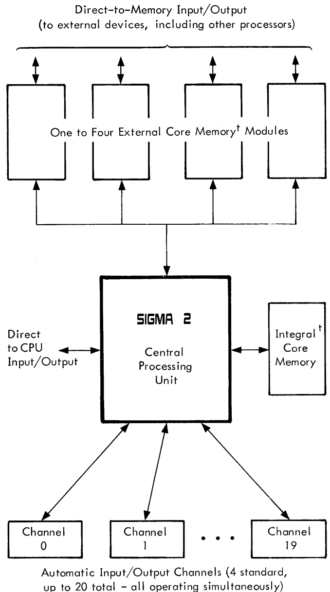
Figure 1. SIGMA 2 System Configuration
